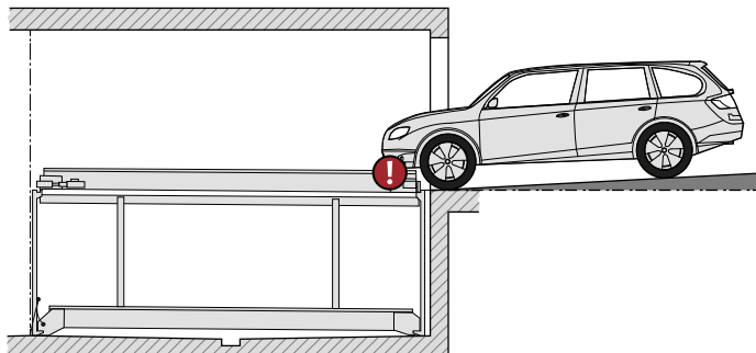
max. 3% slope
